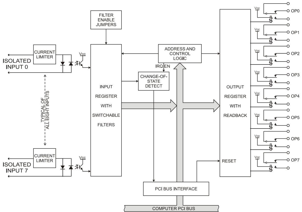
Figure 1-1: Block Diagram
